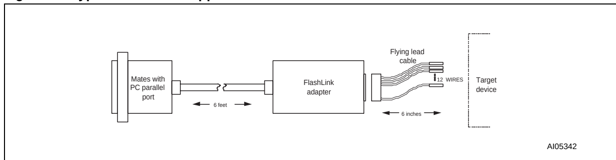
Figure 14. Typical FLASHlink application
